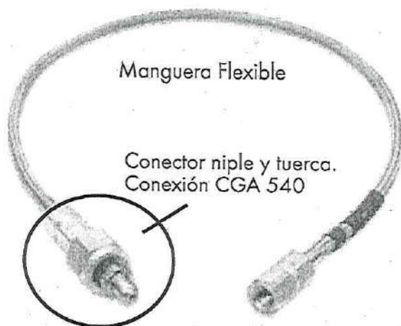
Figura 8.1.5.2 Ilustra la manguera flexible pigtail
